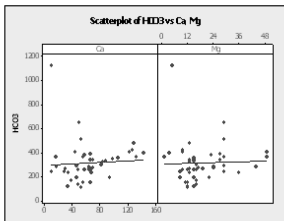
Fig. 5 Correlation of \text{HCO}_3 with Ca and Mg
