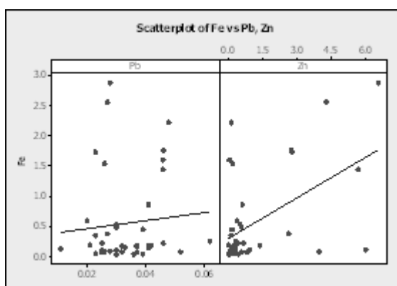
Fig. 8 Correlation of Fe with Pb and Zn
