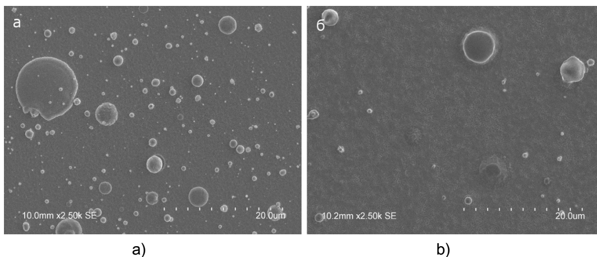
Fig. 2 SEM photographs of substrate surface after 3 min of a treatment (normal field): a) anode potential, b) negative pulsed bias ( \tau=7 \mu\text{s} , f=10^5 p.p.s, U=-2 \text{ kV} ).
