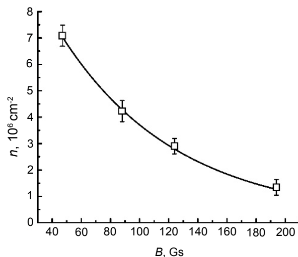
Fig. 5 MP surface number density versus magnetic field strength after 30 sec of coating deposition.
