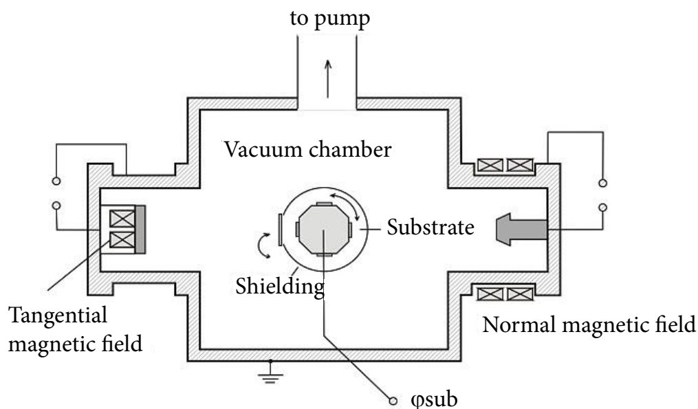
Fig. 1 The experimental installation scheme.
