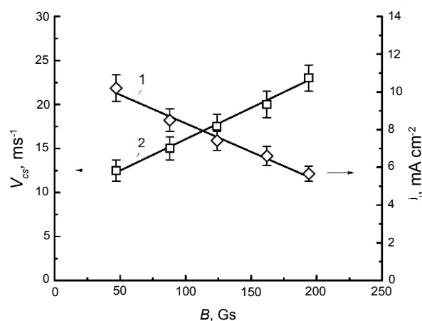
Fig. 4 Ion current density (1) and cathode spot velocity (2) versus tangential magnetic field strength on cathode-to-substrate distance L=24\ \text{cm} .
