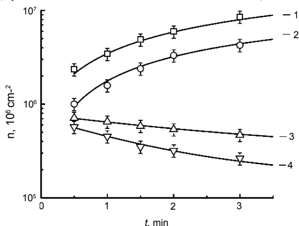
Fig. 3 MP surface number density versus processing time at anode and negative bias potential ( 7\ \mu\text{s} , 10^5 p.p.s, 2 kV): 1-anode potential, normal field; 2-negative bias, normal field; 3-anode potential, tangential field; 4-negative bias, tangential field.
