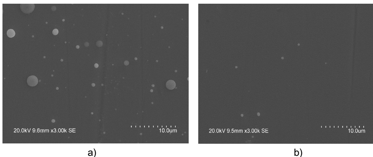
Fig. 6 SEM photographs of substrate surface after 3 min of a treatment (tangential field, 190 Gs): a) anode potential, b) negative pulsed bias ( \tau=7 \mu\text{s} , f=10^5 p.p.s, U=-2 kV).
