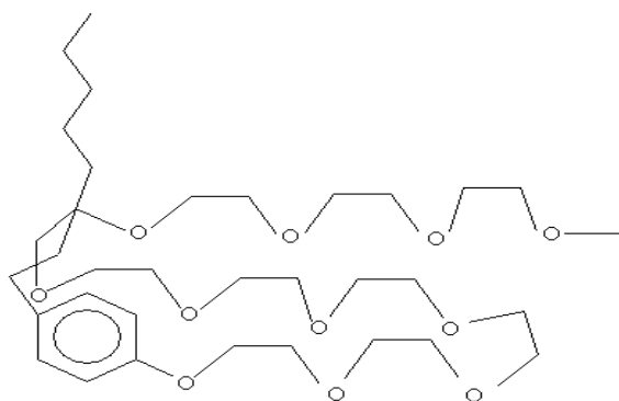
Fig.1 Schematic diagram illustrating arrangement of poly (oxyethylene) units on the water surface
